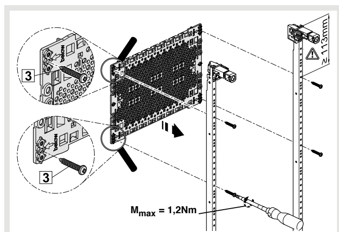
Installation of the UM00M0 plastic plate on the rear of the univers FW mounting rail
