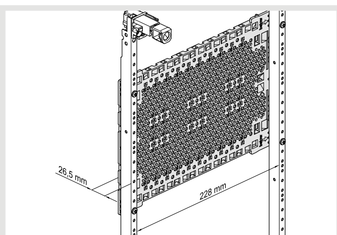
Installation of the UM00M0 plastic plate on the rear of the univers FW mounting rail
