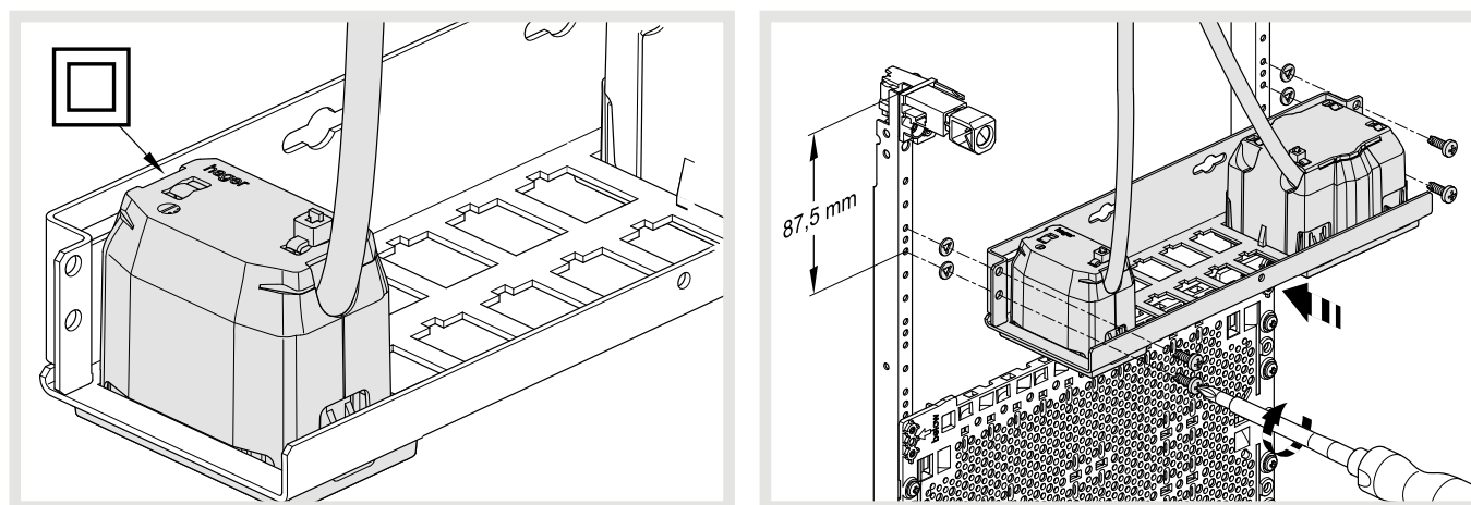
Mounting of the WH37961623Z cover for FLF sockets size I to ensure protection class II
