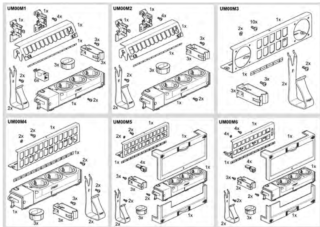
UM00Mx multimedia set overview
