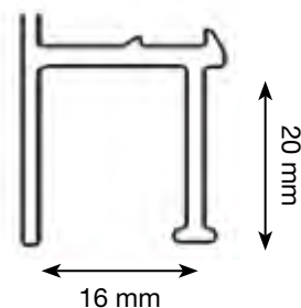
Integrated cable duct in the central area below the mounting rail
