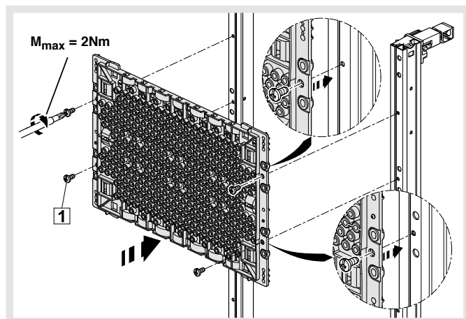
Installation of the UM00M0 plastic plate on the rear of the univers Z mounting rail
