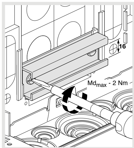
Fixing thick pipes to the plastic bottom part of the cabinet
