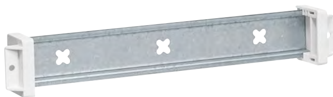
UT22C: 7,5mm DIN rail, insulated, insertable (212 mm length) 1-panel, adjustable depth up to 21 mm
