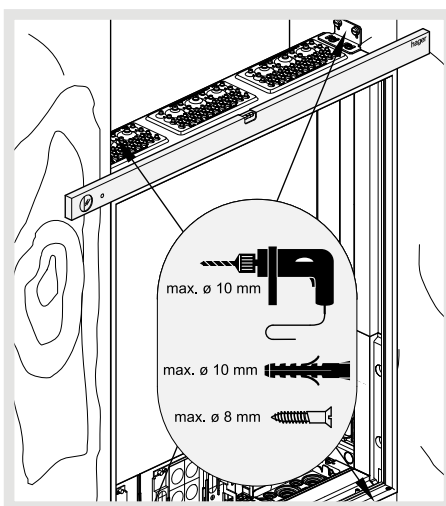
Installation of the FZ900H bracket set for flush and partially recessed installation
