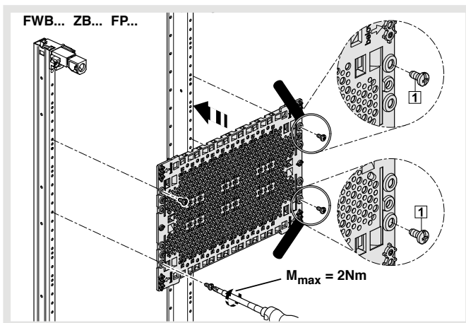
Installation of the UM00M0 plastic plate on the front of the univers Z mounting rail
