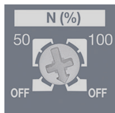
Neutral protection dial LSI trip unit
