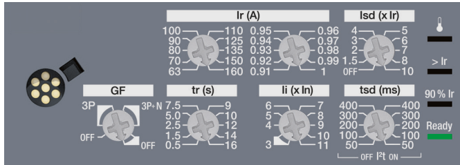
Trip unit LSIG for 3 poles
