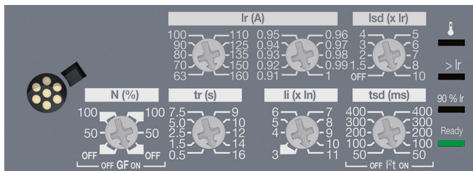
Trip unit LSIG for 4 poles
