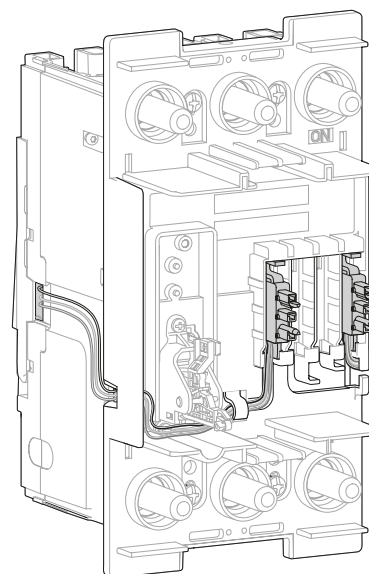
P250 Plug-in circuit breaker adaptor fitted with internal auxiliaries
