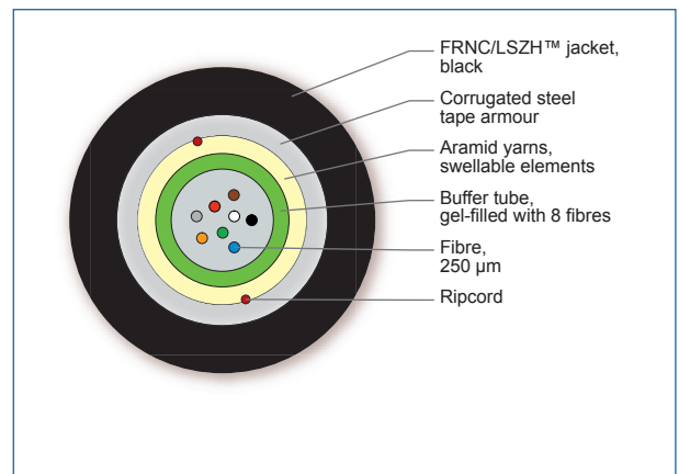
Cross Section of Order Number: 008TEY-13188A2G
